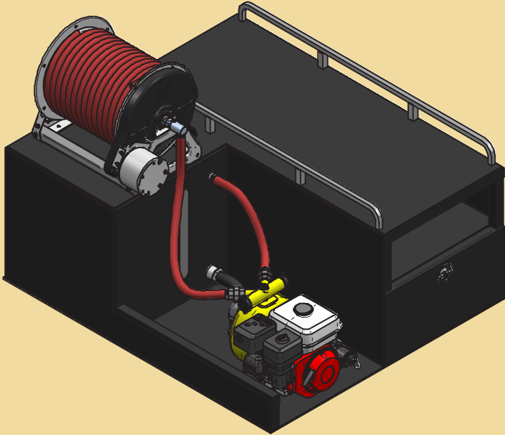
70 GALLON SKID W/ ELECTRIC HOSE REEL SHOWN
