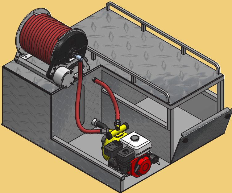
70 GALLON SKID W/ ELECTRIC HOSE REEL SHOWN
